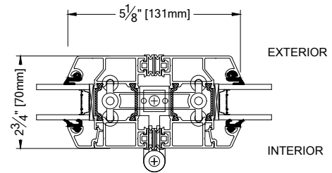
Roller Point
