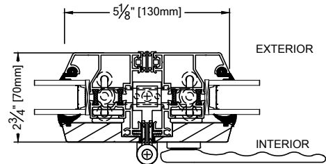
Roller Point
